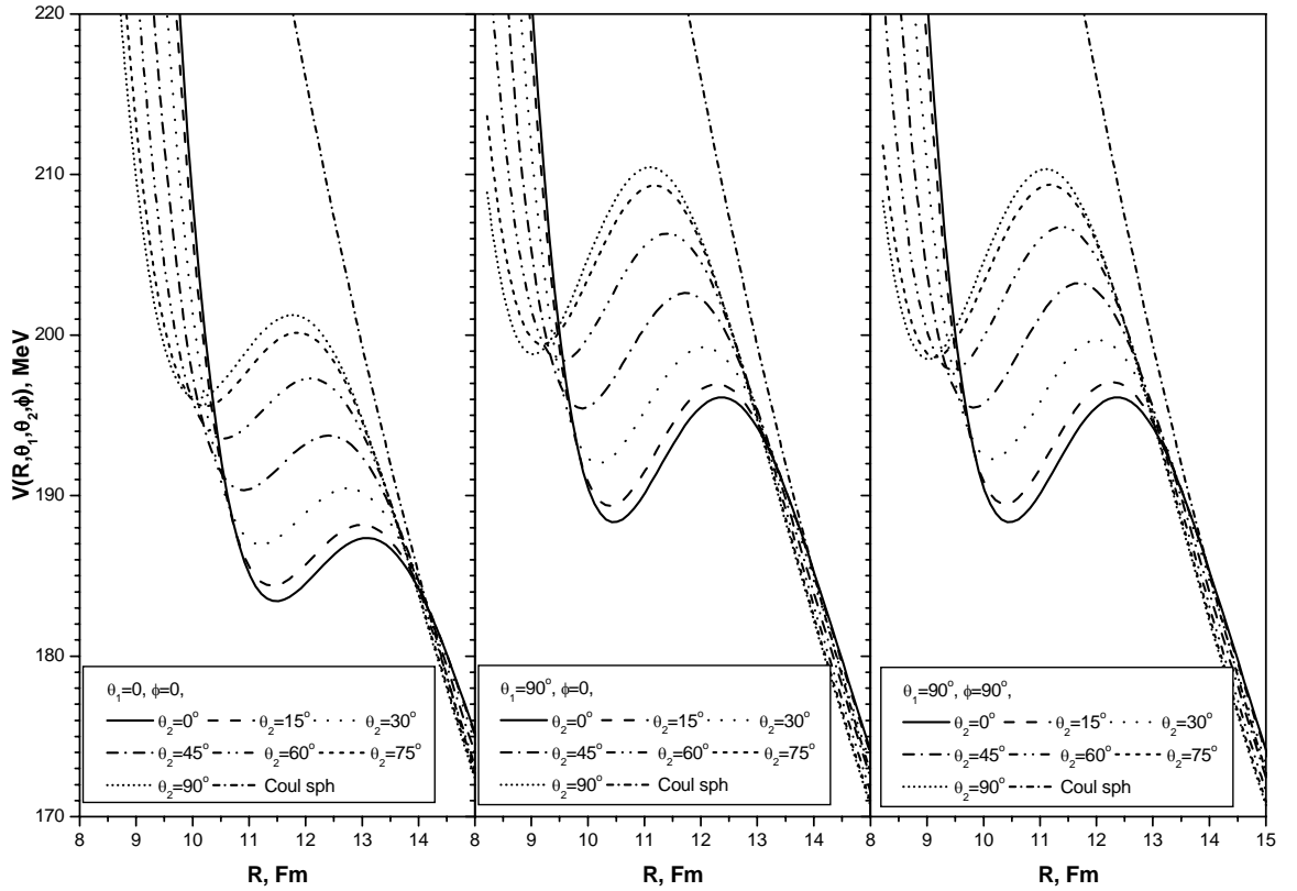
Fig. 2. Potentials between ^{64}\text{Zn} + ^{150}\text{Nd} for various orientation of both ^{64}\text{Zn} and ^{150}\text{Nd} . The Coulomb potential between these nuclei, when shapes of both nuclei are considered spherical, is also presented for comparison.
