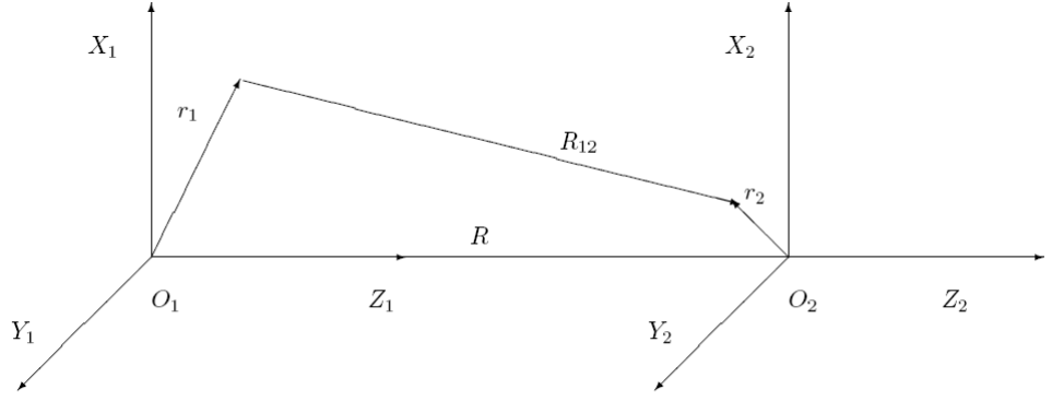
Fig. 1. The coordinate systems related to the mass centers of corresponding nuclei.
