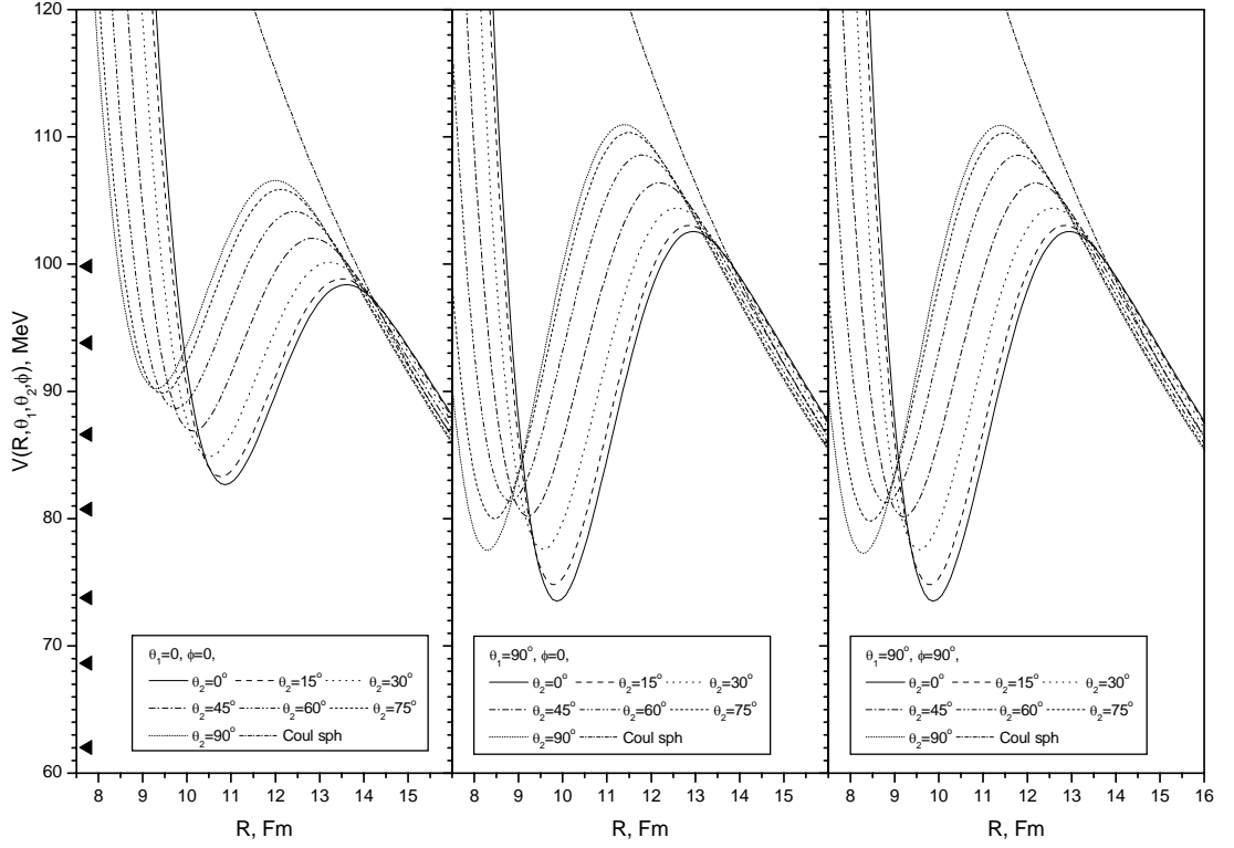
Fig. 4. The nucleus-nucleus potentials for the system ^{22}\text{Ne} + ^{248}\text{Cm} for various orientations of both ^{22}\text{Ne} and ^{248}\text{Cm} . The Coulomb potential between these nuclei, when both nuclei are considered spherical, is also presented for comparison. The ground-state Q-values are indicated by the lowest triangles at the left vertical axes. The other 6 triangles mark, respectively, the thresholds for the emission of 1, 2, 3, 4, 5 and 6 neutrons.
