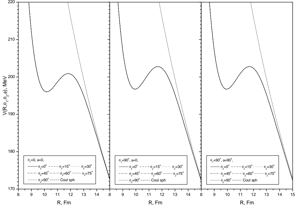
Fig. 3. Potentials between ^{70}\text{Zn} + ^{144}\text{Nd} for various orientation of both ^{70}\text{Zn} and ^{144}\text{Nd} . The Coulomb potential between these nuclei, when both nuclei are considered spherical, is also presented for comparison.
