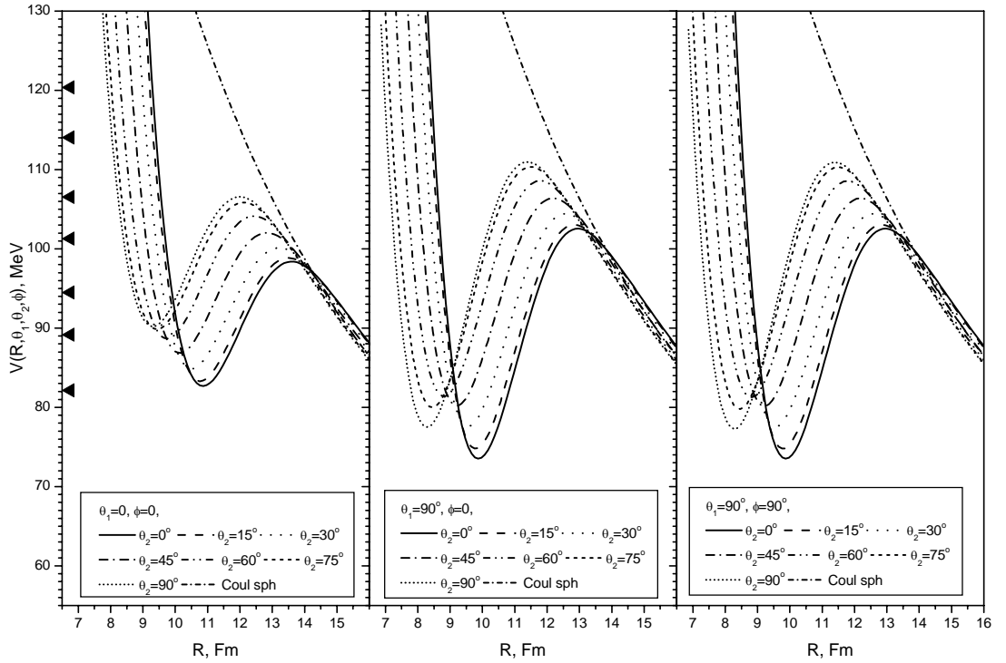
Fig. 5. The nucleus-nucleus potentials for the system ^{26}\text{Mg} + ^{248}\text{Cm} for various orientations of both ^{26}\text{Mg} and ^{248}\text{Cm} . The notations are similar to the ones in Fig. 4.
