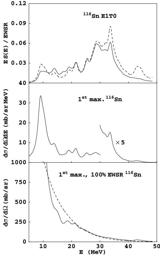
Fig. 2. Reconstruction of the ISGDR EWSR in ^{116}\text{Sn} from the inelastic \alpha -particle cross sections. Middle panel: maximum double differential cross section obtained from \rho_t (RPA). Lowest panel: maximum cross section ( 0^\circ degrees) obtained with \rho_{coll} (dashed line) and \rho_t (solid line) normalized to 100 % of the EWSR. Upper panel: The solid and dashed lines are the ratios of the middle panel curve with the solid and dashed lines of the lower panel, respectively (taken from Ref. [33]).
