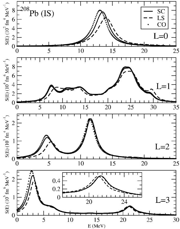
Fig. 1. Isoscalar strength functions of ^{208}\text{Pb} for L=0-3 multi-polarities are displayed. SC (full line) corresponds to the fully self-consistent calculation where LS (dashed line) and CO (open circle) represent the calculations without the ph spin-orbit and Coulomb interactions in the RPA, respectively. The Skyrme interaction SGII [52] was used (taken from Ref. [48]).
